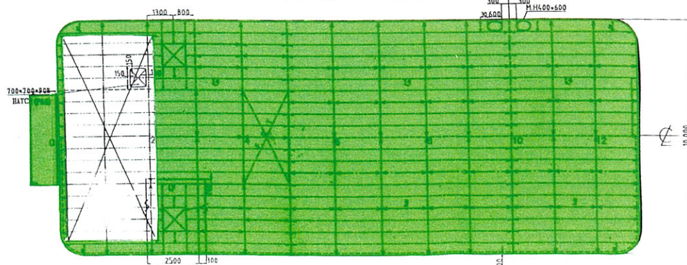
BOTT PLAN BOTT FLOOR & KEELSON 8*300+9*100FB BOTT LONGI. 100*75*71A
